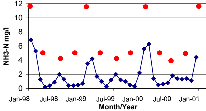
Figure 17. Average monthly NH3 in Granger effluent.
