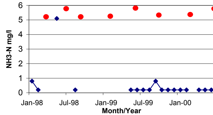
Figure 20. Average monthly NH3 in Lake Park effluent.
