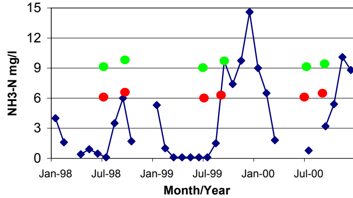
Figure 15. Average monthly NH3 in Norway effluent.
