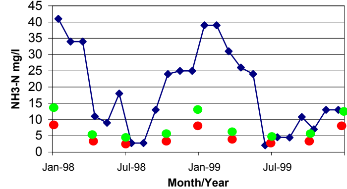
Figure 18. Average monthly NH3 in Chelsea Effluent.
