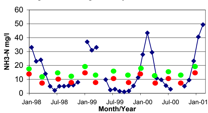
Figure 19. Average monthly NH3 in Laurel effluent.
