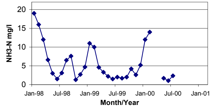
Figure 18. Average monthly NH3 in Chelsea Effluent.
