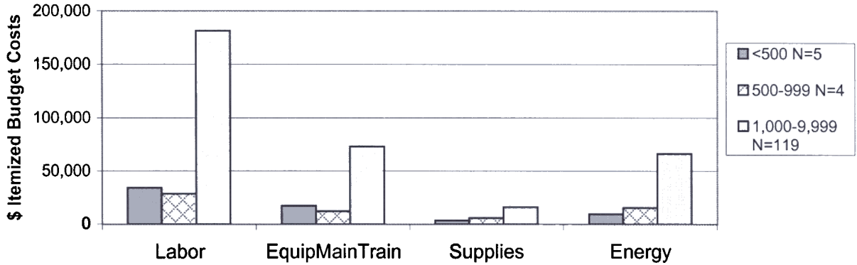
Figure WW10-1. Mean 1999 - 2000 annual itemized budget costs for Iowa wastewater treatment systems with activated sludge.
