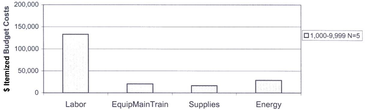
Figure WW13-1. Mean 1999 - 2000 annual itemized budget costs for Iowa wastewater treatment systems with rotating biological contactor.
