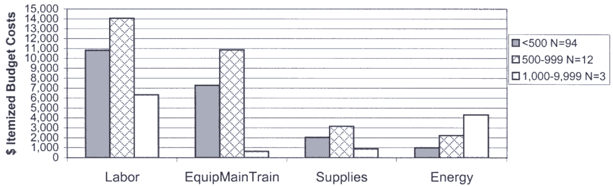
Figure WW14-1. Mean 1999 - 2000 annual itemized budget costs for Iowa wastewater treatment systems with nonaerated facultative lagoon.
