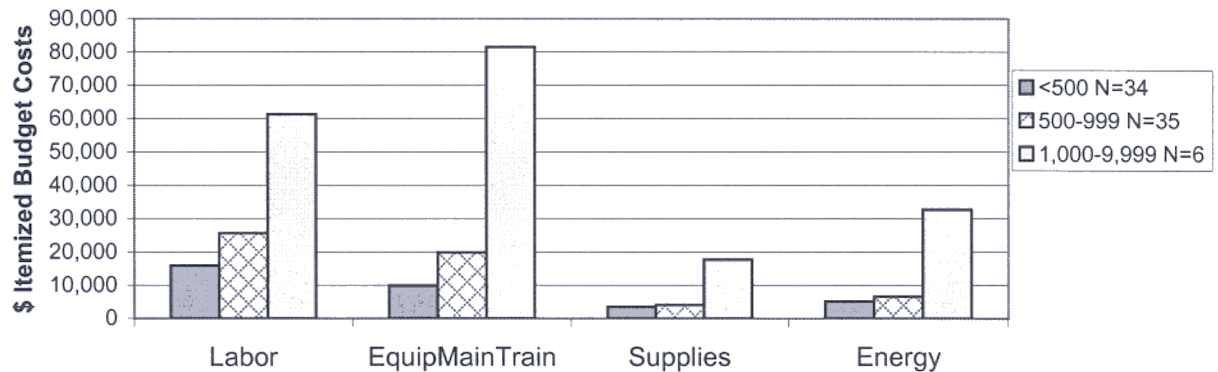
Figure WW15-1. Mean 1999 - 2000 annual itemized budget costs for Iowa wastewater treatment systems with aerated facultative lagoon.
