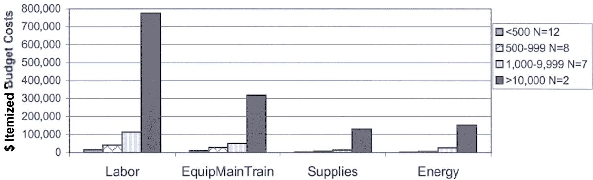
Figure WW11-1. Mean 1999 - 2000 annual itemized budget costs for Iowa wastewater treatment systems with trickling filters.
