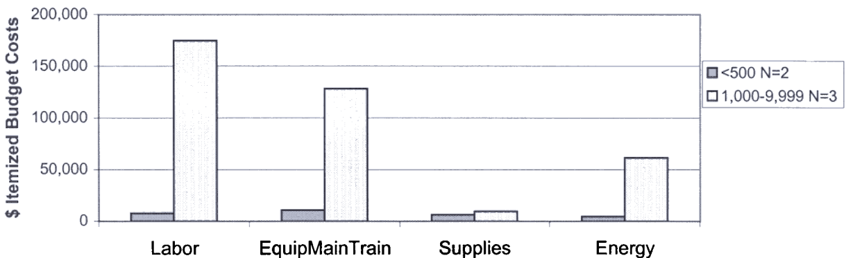
Figure WW12-1. Mean 1999 - 2000 annual itemized budget costs for Iowa wastewater treatment systems with activated sludge & trickling filters.
