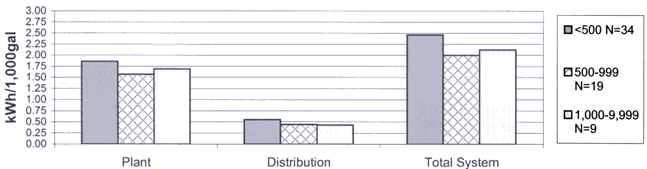
Figure WW7-3. Mean 1999 - 2000 kilowatt-hr/1,000 gal consumed to treat surveyed Iowa wastewater treatment systems with aerated facultative lagoon.
