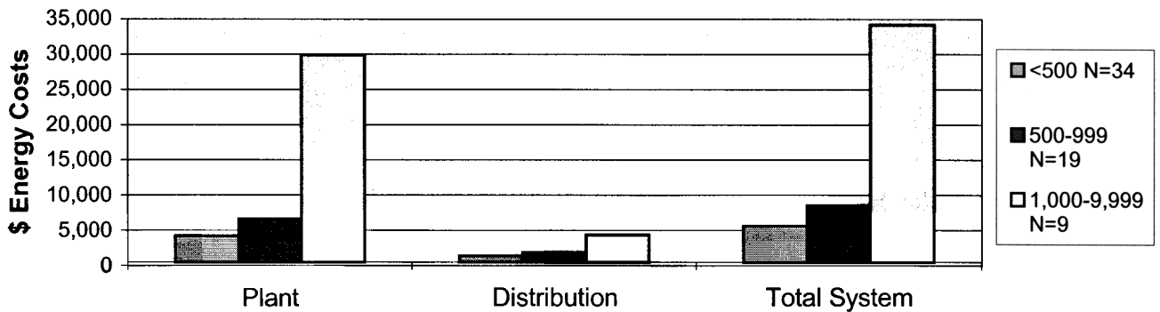
Figure WW7-2. Mean 1999 - 2000 energy costs for surveyed Iowa wastewater treatment systems with aerated facultative lagoon.
