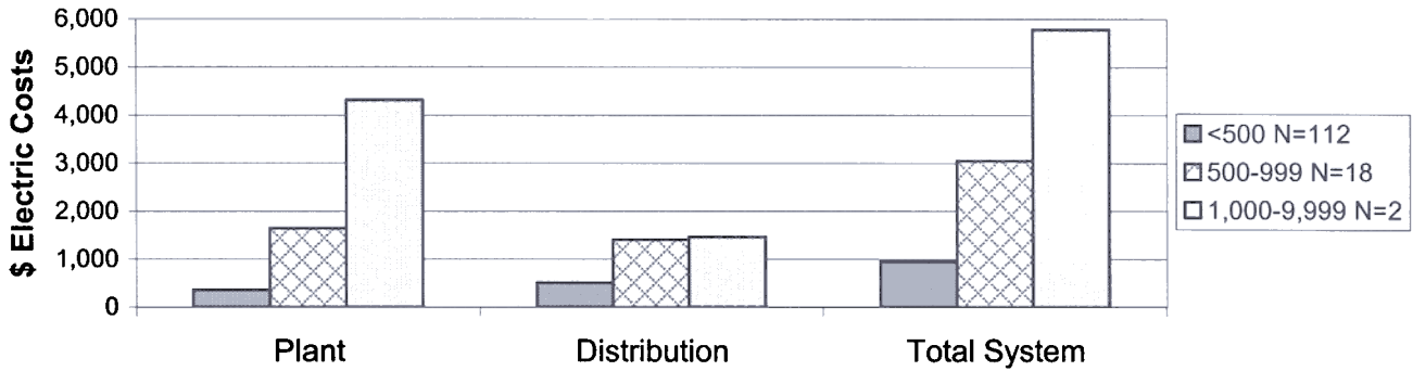
Figure WW6-1. Mean 1999 - 2000 electric costs for surveyed Iowa wastewater treatment systems with nonaerated facultative lagoon.
