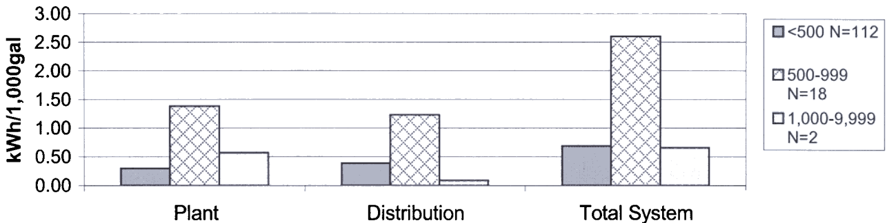
Figure WW6-3. Mean 1999 - 2000 kilowatt-hr/1,000 gal consumed to treat surveyed Iowa wastewater treatment systems with nonaerated facultative lagoon.
