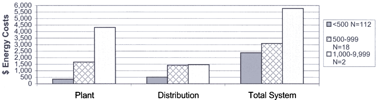
Figure WW6-2. Mean 1999 - 2000 energy costs for surveyed Iowa wastewater treatment systems with nonaerated facultative lagoon.
