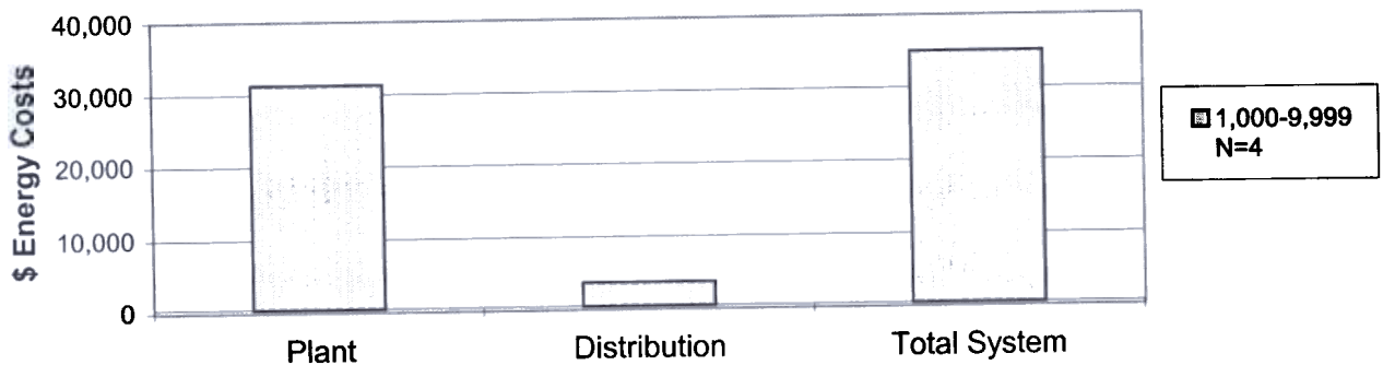
Figure WW5-2. Mean 1999 - 2000 energy costs for surveyed Iowa wastewater treatment systems with rotating biological contactor.
