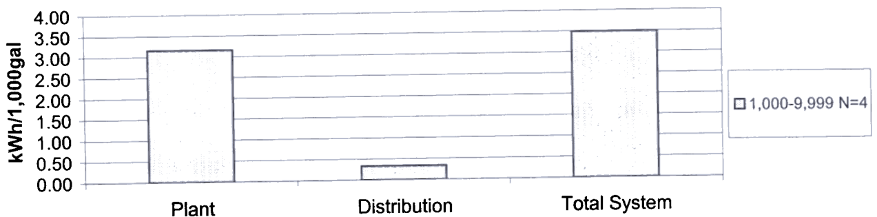
Figure WW5-3. Mean 1999 - 2000 kilowatt-hr/1,000 gal consumed to treat surveyed Iowa wastewater treatment systems with rotating biological contactor.
