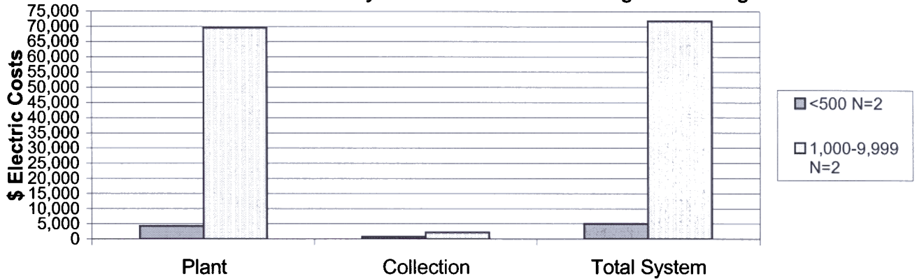
Figure WW4-1. Mean 1999 - 2000 electric costs for surveyed Iowa wastewater treatment systems with activated sludge & trickling filter.
