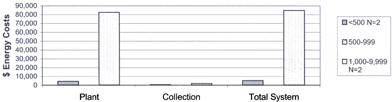
Figure WW4-2. Mean 1999 - 2000 energy costs for surveyed Iowa wastewater treatment systems with activated sludge & trickling filter.
