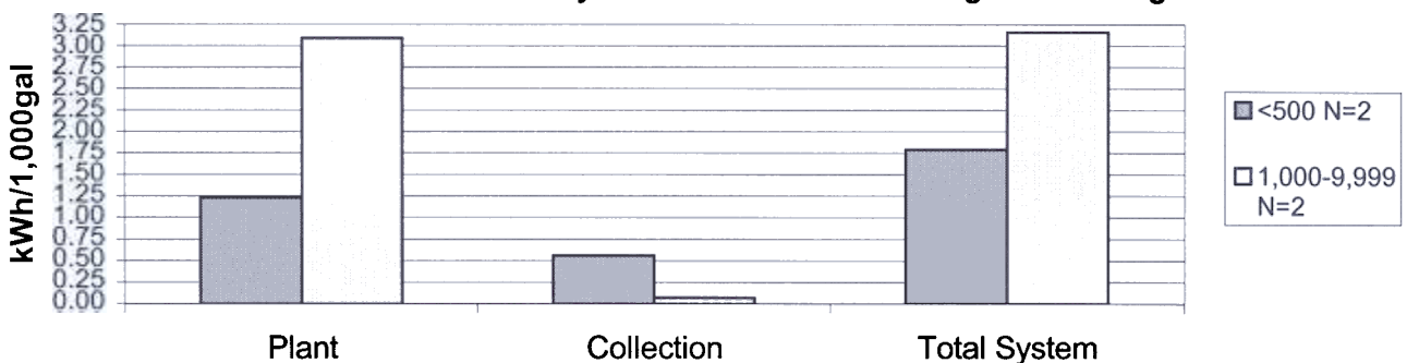
Figure WW4-3. Mean 1999 - 2000 kilowatt-hr/1000 gal consumed to treat surveyed Iowa wastewater treatment systems with activated sludge & trickling filter.
