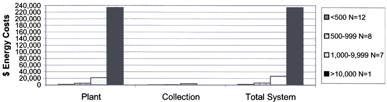
Figure WW3-2. Mean 1999 - 2000 energy costs for surveyed Iowa wastewater treatment systems with trickling filter.
