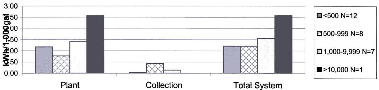
Figure WW3-3. Mean 1999 - 2000 kilowatt-hr/1,000 gal consumed to treat surveyed Iowa wastewater treatment systems with trickling filter.
