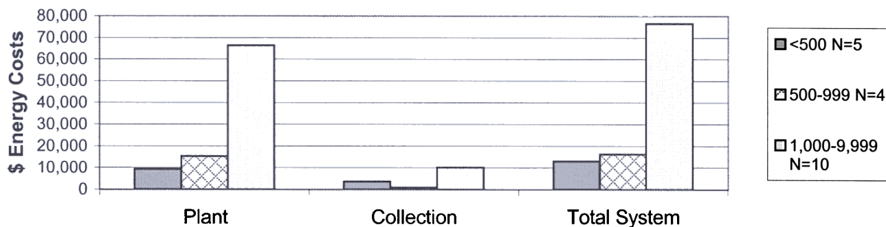
Figure WW2-2. Mean 1999 - 2000 energy costs for surveyed Iowa wastewater treatment systems with activated sludge.
