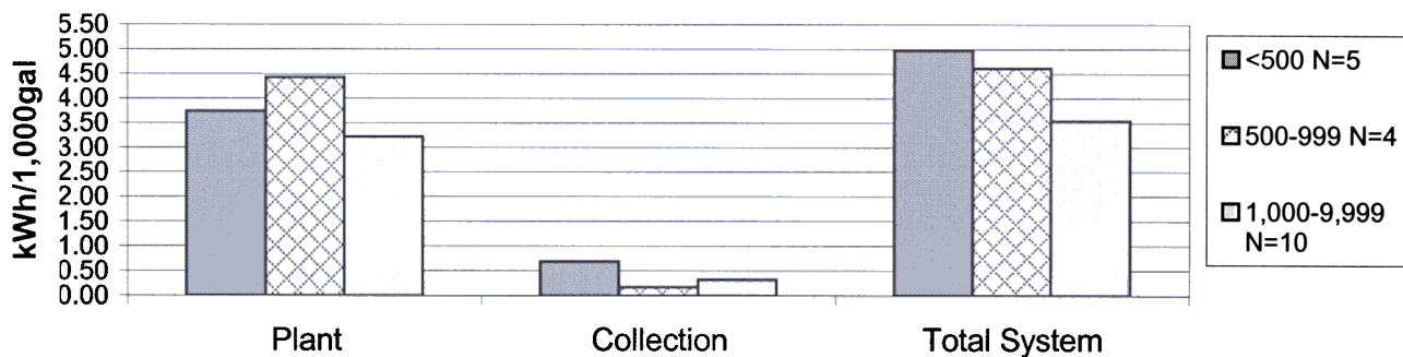
Figure WW2-3. Mean 1999 - 2000 kilowatt-hr/1,000 gal consumed to treat surveyed Iowa wastewater treatment systems with activated sludge.
