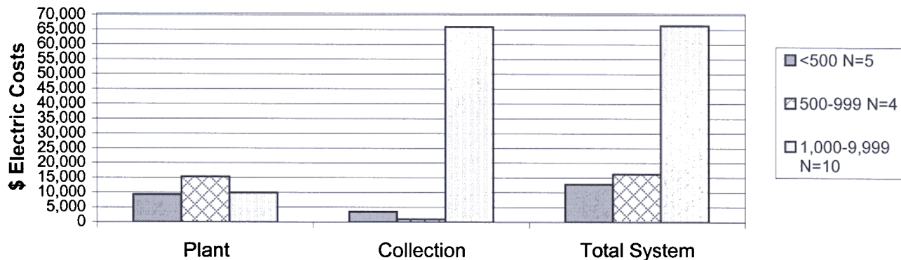
Figure WW2-1. Mean 1999 - 2000 electric costs for surveyed Iowa wastewater treatment systems with activated sludge.
