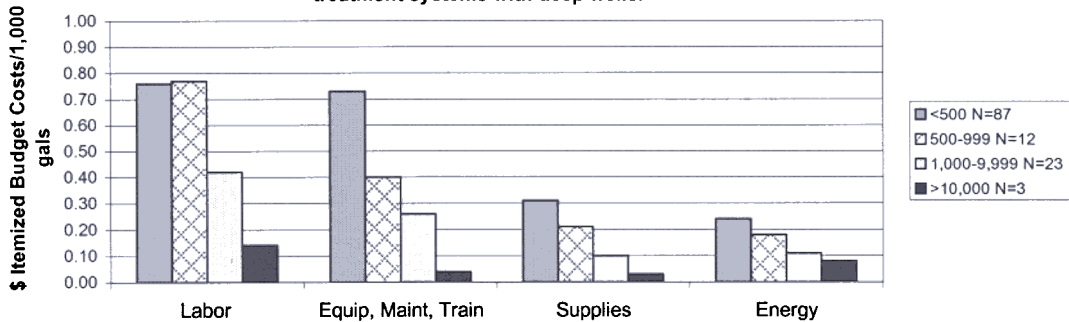
Figure W16-1. Mean 1999 - 2000 itemized budget costs/1,000 gallons for Iowa water treatment systems with deep wells.
