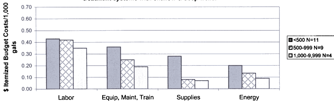
Figure W17-1. Mean 1999 - 2000 itemized budget costs/1,000 gallons for Iowa water treatment systems with shallow & deep wells.
