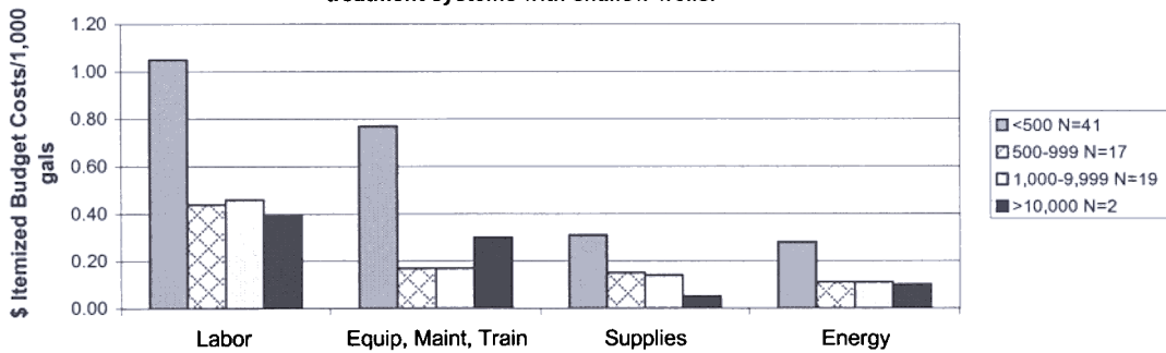
Figure W15-1. Mean 1999 - 2000 itemized budget costs/1,000 gallons for Iowa water treatment systems with shallow wells.
