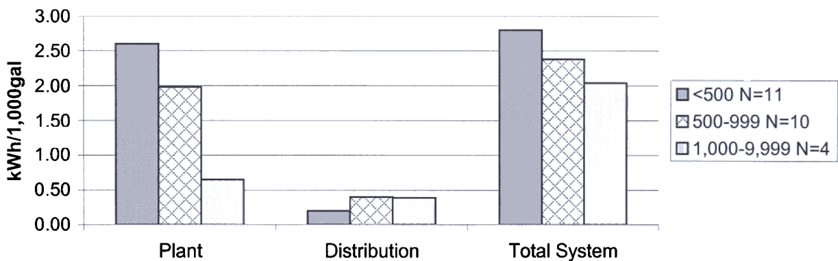
Figure W5-3. Mean 1999 - 2000 kilowatt-hr/1,000 gal consumed to treat water for Iowa shallow and deep wells.
