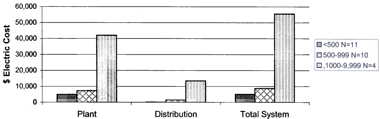
Figure W5-1. Mean 1999 - 2000 electric costs for Iowa water treatment systems with shallow and deep wells.
