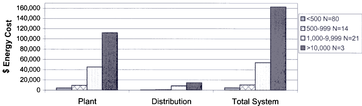
Figure W4-2. Mean 1999 - 2000 energy costs for Iowa water treatment systems with deep wells.
