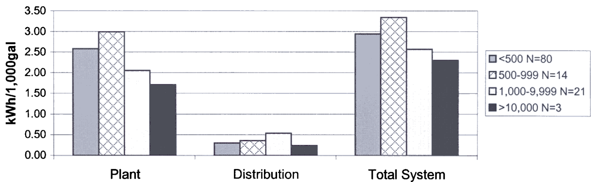
Figure W4-3. Mean 1999 - 2000 kilowatt-hr/1,000 gal. consumed to treat water for Iowa deep wells.
