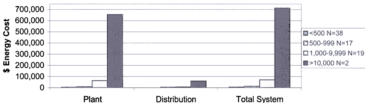
Figure W3-2. Mean 1999 - 2000 energy costs for Iowa water treatment systems with shallow wells.
