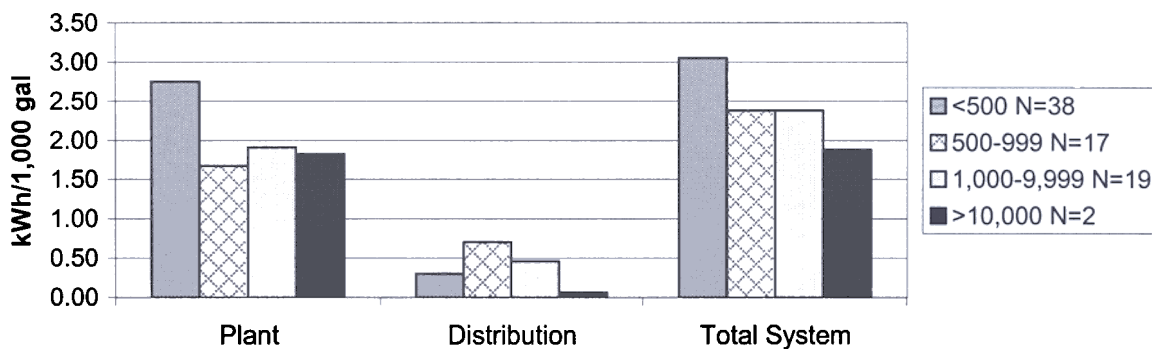
Figure W3-3. Mean 1999 - 2000 kilowatt-hr/1,000 gal. consumed to treat water for Iowa shallow wells.
