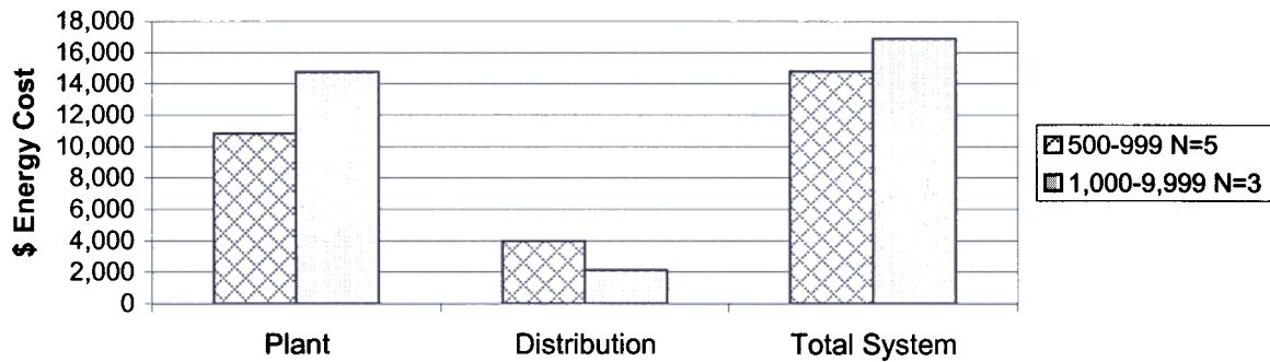
Figure W2-2. Mean 1999 - 2000 total energy cost for Iowa water treatment systems with surface water.
