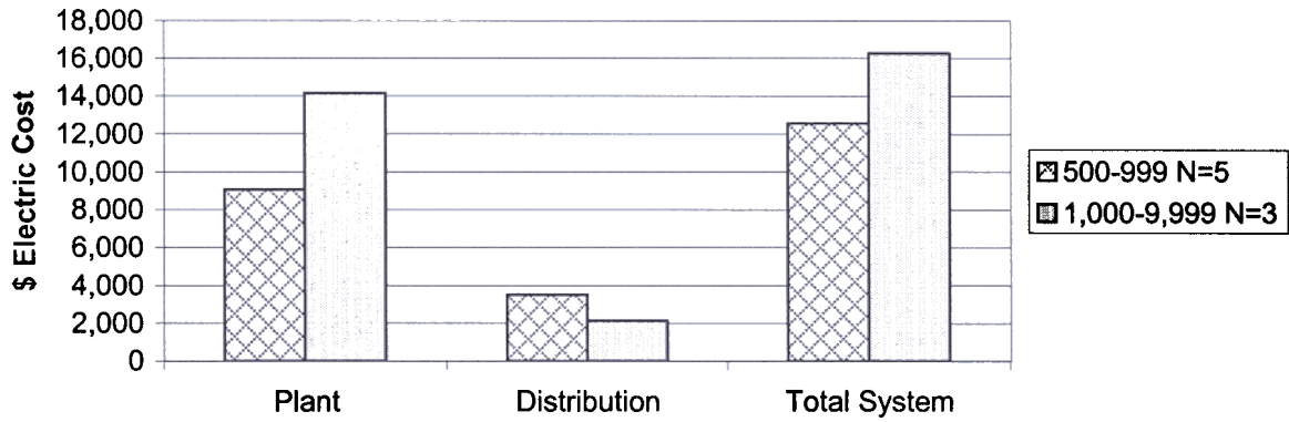
Figure W2-1. Mean 1999 - 2000 electric cost for Iowa water treatment systems with surface water.
