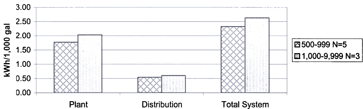
Figure W2-3. Mean 1999 - 2000 kilowatt-hr/1,000 gal. consumed to treat water for Iowa surface water.
