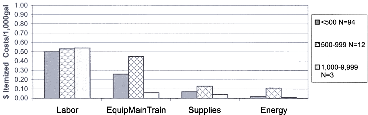
Figure WW23-1. Mean 1999 - 2000 annual itemized budget costs/1,000 gal for Iowa wastewater treatment systems with aerated facultative lagoon.
