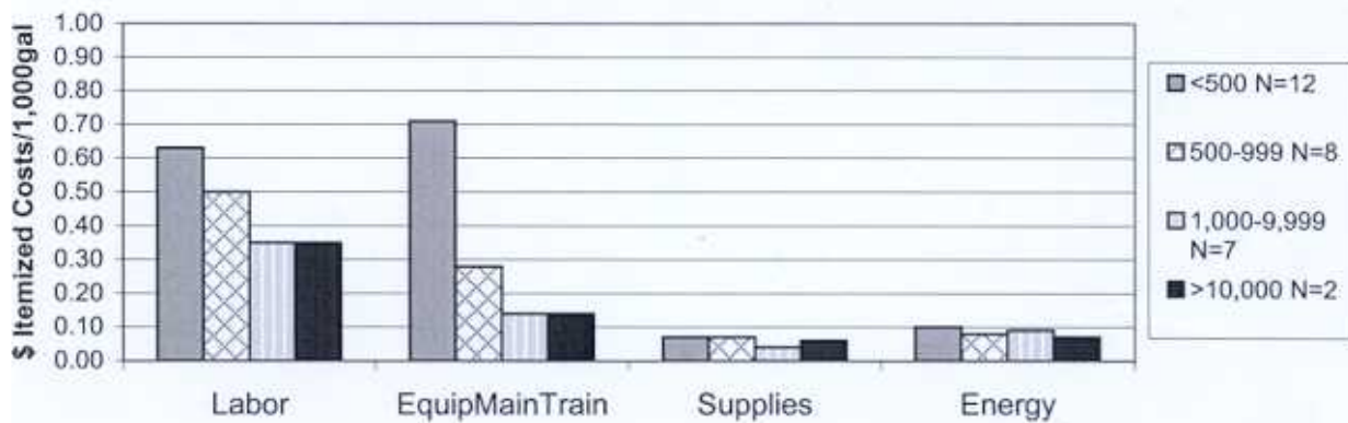
Figure WW19-1. Mean 1999 - 2000 annual itemized budget costs/1,000 gal for Iowa wastewater treatment systems with trickling filters.
