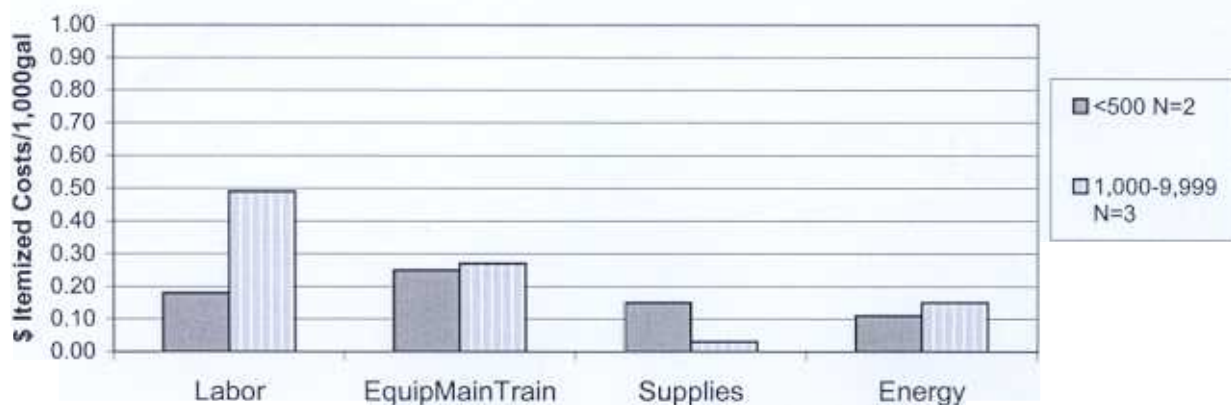
Figure WW20-1. Mean 1999 - 2000 annual itemized budget costs/1,000 gal for Iowa wastewater treatment systems with activated sludge and trickling filters.
