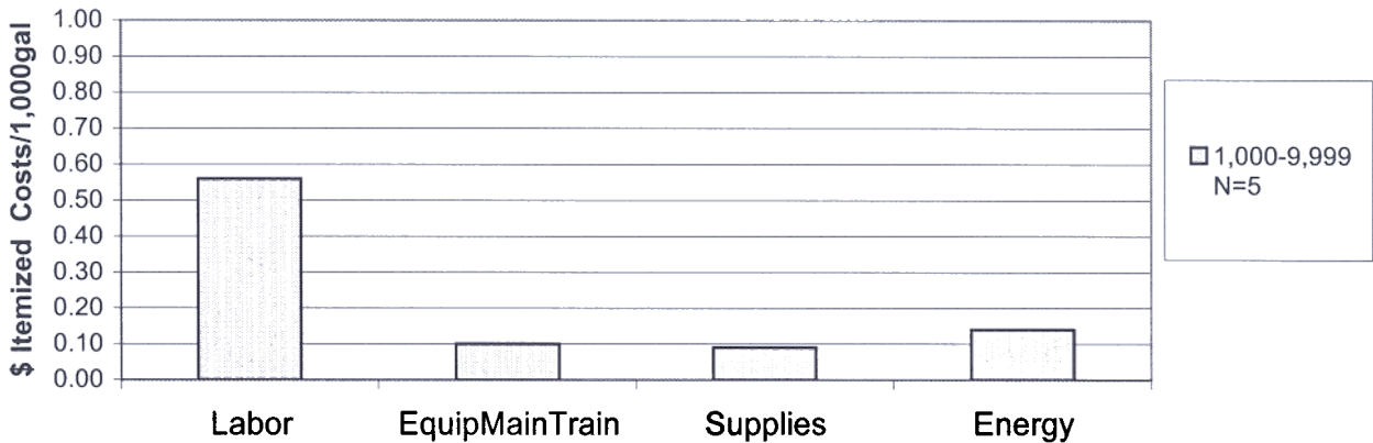
Figure WW21-1. Mean 1999 - 2000 annual itemized budget costs/1,000 gal for Iowa wastewater treatment systems with rotating biological contactor.
